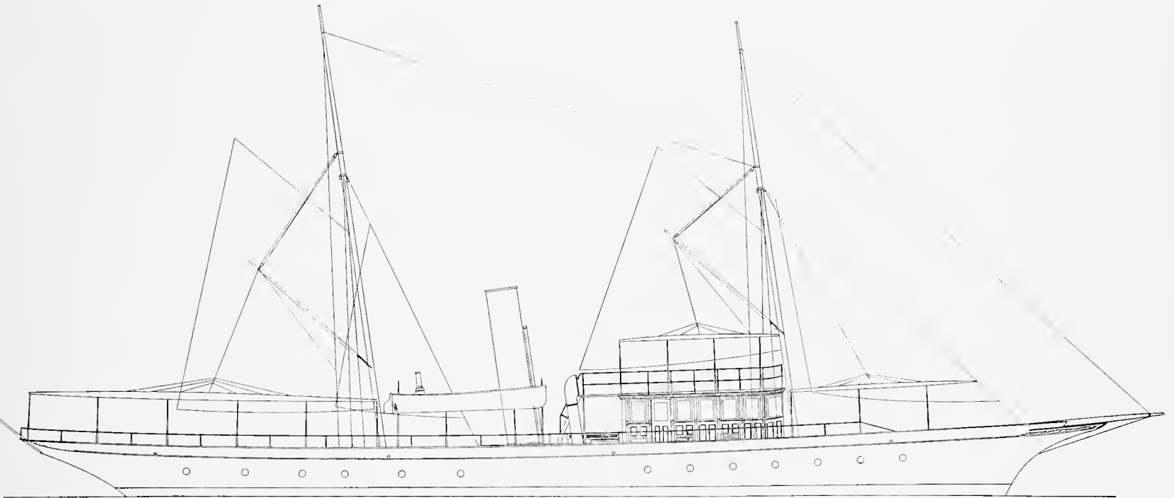
SHEAR PLAN OF THE COMPOSITE STEAM YACHT ALCEDO.
